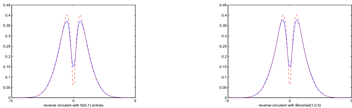
Figure 2: (i) (left) dashed line represents the LSD of the reverse circulant matrix with entries x_t = 0.3\epsilon_t + \epsilon_{t+1} + 0.5\epsilon_{t+2} where \{\epsilon_i\} i.i.d. N(0, 1) . The continuous line represents the kernel density estimate of ESD of the same matrix of order 5000 \times 5000 with same \{x_t\} . (ii) same graphs with centered and scaled Binomial(1, 0.5).
