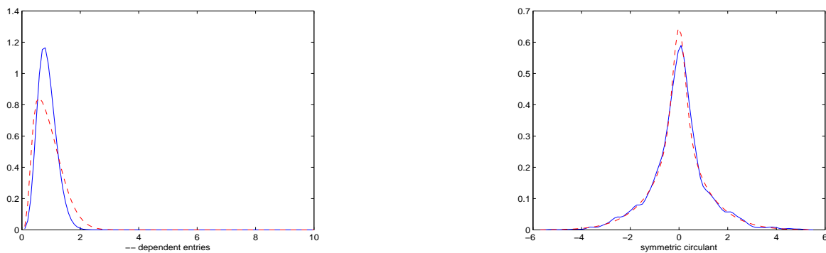
Figure 1: (i) (left) dashed line represents the density of F_2 when f(\omega) = \frac{1}{2\pi}(1.25 + \cos x) and the continuous line represents the same with f = \frac{1}{2\pi} . (ii) (right) dashed line represents the LSD of symmetric circulant matrix with entries x_t = 0.3\epsilon_t + \epsilon_{t+1} + 0.5\epsilon_{t+2} where \{\epsilon_i\} i.i.d. N(0, 1) and the continuous line represents the kernel density estimate of the ESD of the same matrix of order 5000 \times 5000 and same \{x_t\} .
