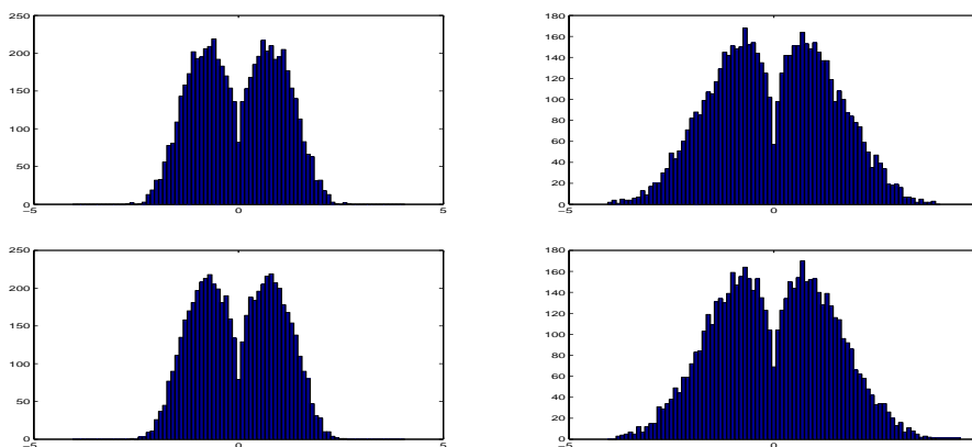
Figure 2: Histograms of the ESD of 15 realizations of the Hankel matrix (left) and the balanced Toeplitz matrix (right) of order 400 with standardized Normal(0, 1) (top row), and Bernoulli(0.5) (bottom row) entries.
