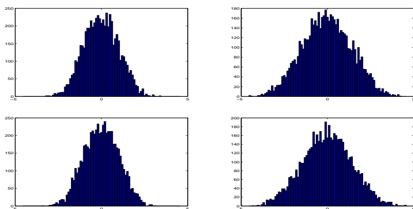
Figure 1: Histograms of the ESD of 15 realizations of the Toeplitz matrix (left) and the balanced Toeplitz matrix (right) of order 400 with standardized Normal(0, 1) (top row), and Bernoulli(0.5) (bottom row) entries.
