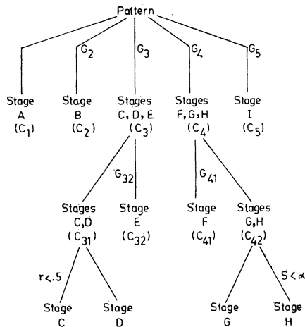
Fig. 3. Three-stage hierarchical classification scheme.
