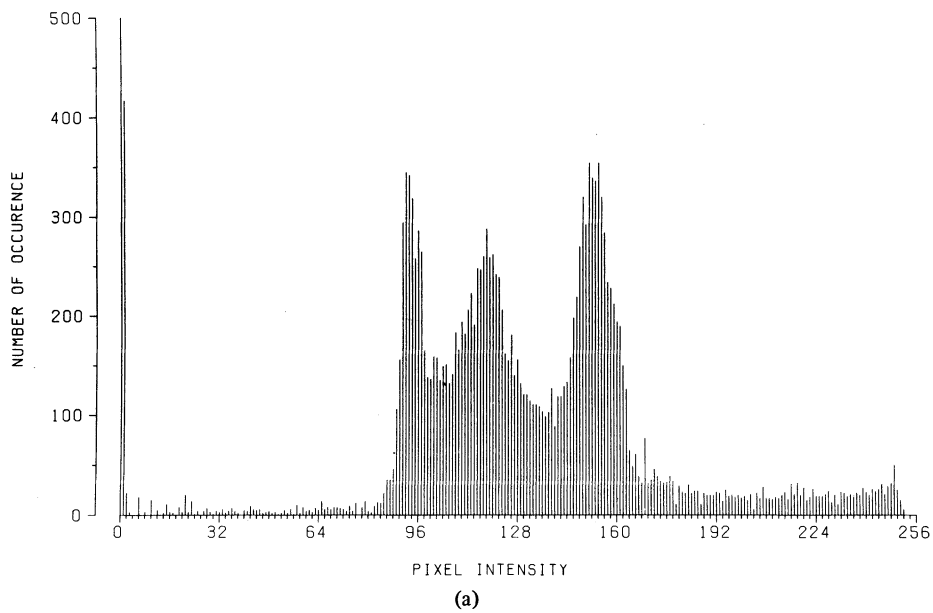
Fig. 6. Histogram of input image.
