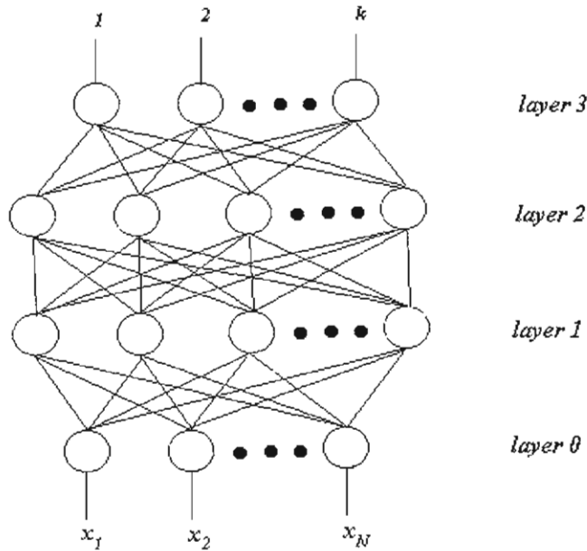
Figure 2. Multilayer perceptron
