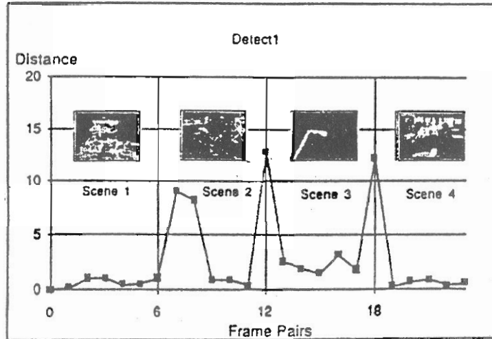
Fig. 4 Distance between successive frames with feature set (entropy, compactness, length/height)
