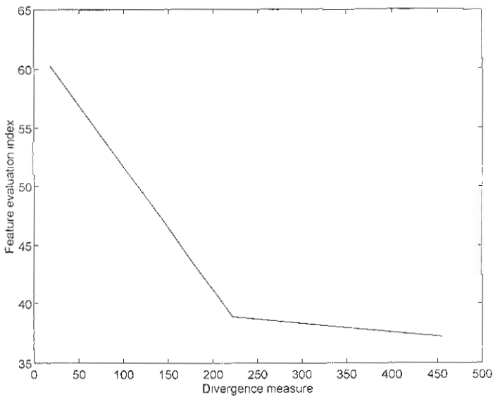
Fig. 6. Graphical representation of the relationship between feature evaluation index and divergence measure for Iris data.
