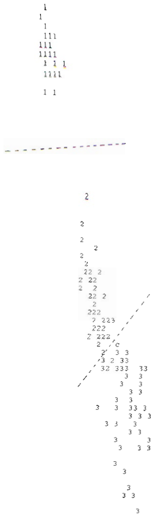
Fig. 5. Scatterplot, using features 3 and 4, of Iris data "1," "2," and "3" indicate patterns belonging to classes 1, 2, and 3, respectively
