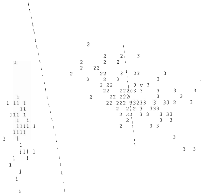
Fig. 4. Scatterplot, using features 2 and 3, of Iris data. "1," "2," and "3" indicate patterns belonging to classes 1, 2, and 3, respectively.
