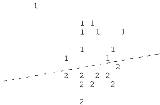
Fig. 2. Scatterplot, using features 1 and 2, of the four-dimensional synthetic data. "1" and "2" indicate patterns belonging to classes 1 and 2, respectively.
