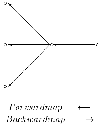
Fig. 1: Sketch of Forward map and backward maps
