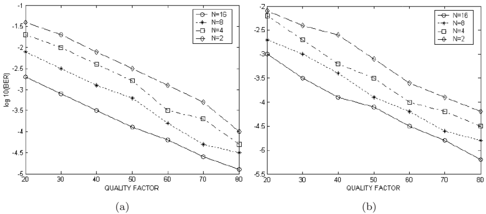
Fig. 17. BER performance of different N -values for (a) M = 4 ; (b) M = 5 under JPEG 2000 compression.
