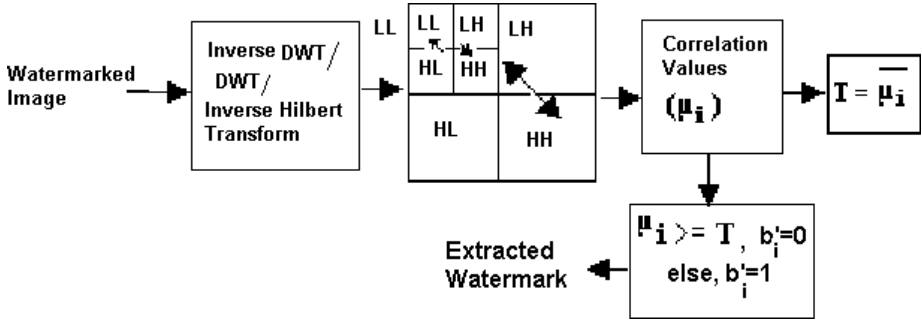
Fig. 5. Block diagram of watermark deiding using DWT.
