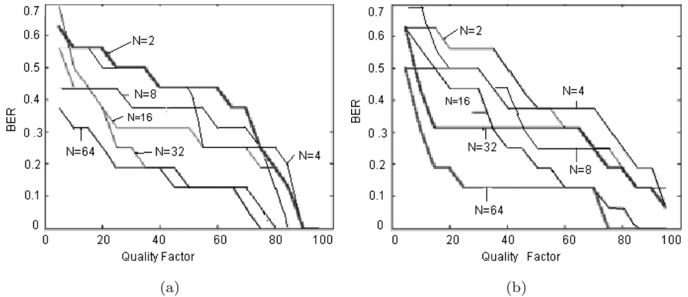
Fig. 15. Effect of N -ary modulation on detection reliability (a) JPEG compression, and (b) JPEG 2000 compression.
