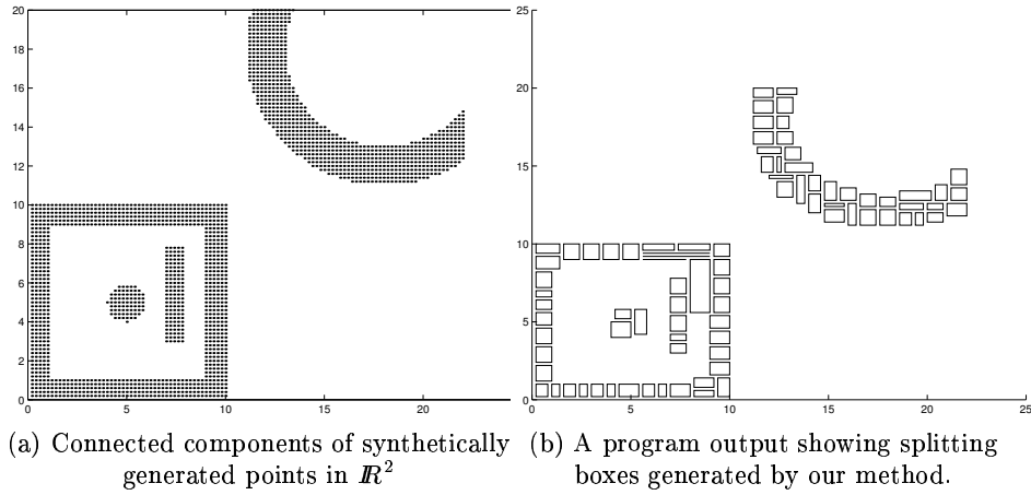
Fig. 2. An example of adaptive clustering and space partitioning.
