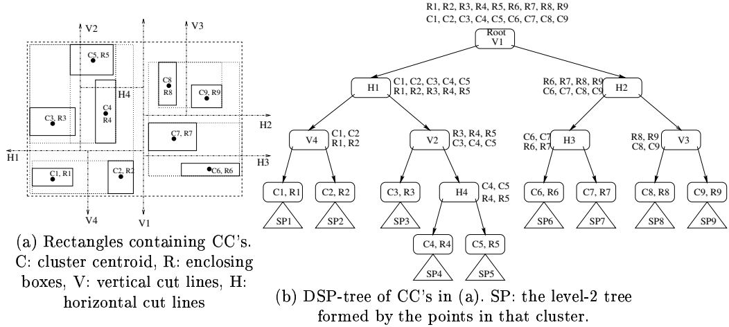
Fig. 1. An example of space partitioning and indexing structure in 2D.
