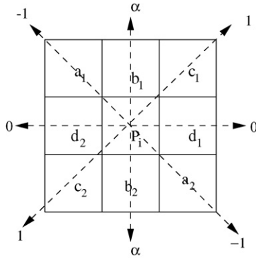
Fig. 3. 3 \times 3 neighborhood of a pixel.
