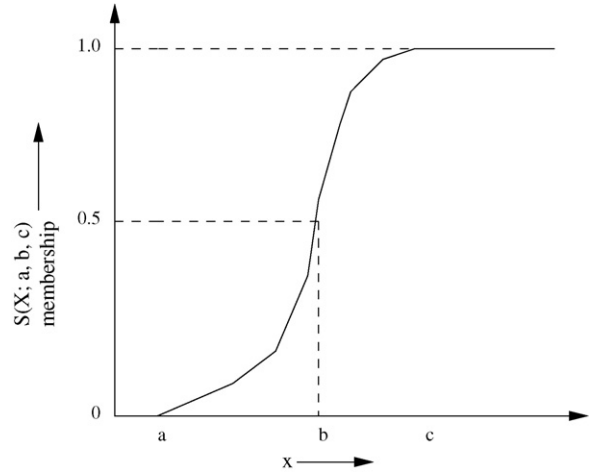
Fig. 1. S-type membership function.
