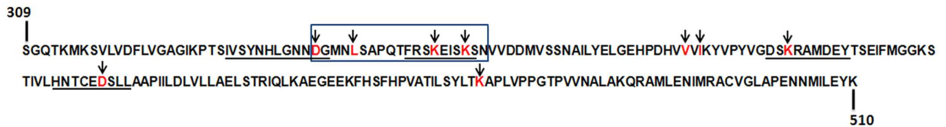
Fig 4. Construction of OsMIPS deletion/substitution mutants. (A) Sequence alignment comparison study of OsMIPS, ScMIPS and A/MIPS through MultAlin. Yellow arrow signifies the NAD-binding residues; red oval signifies the substrate binding residues in ScMIPS; and black triangle active site residues in A/MIPS. Numbering of amino acids presented at the bottom line is with respect to ScMIPS sequence and numbering of amino acids presented at the top line is with respect to A/MIPS sequence. (B) Diagrammatic representation of the generated site-specific deletion mutants of OsMIPS. Black arrows point to the amino acid residue (in red font) has been deleted and/or replaced by alanine from the wild-type OsMIPS following the procedure described in Materials and Methods section. The box represents the “core catalytic domain” and the four evolutionarily conserved blocks within the catalytic site are underlined.
